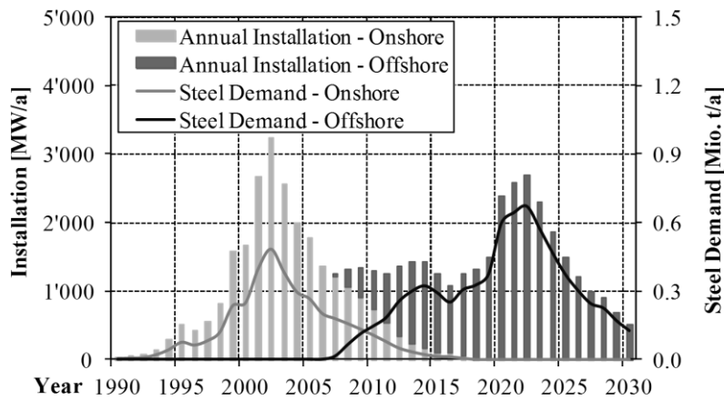
Figure 1: Cumulated capacity and annual steel demand for the German wind energy market (Dewi (2009))
