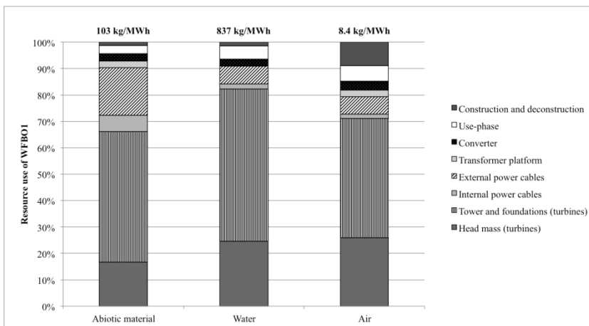
Figure 2: Resource use of WFBO1 for the subsystems wind farm (turbines, internal cables), grid connection (transformer platform and converter, external cables), use phase, construction and deconstruction
